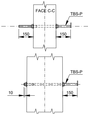
DETAIL D - PERMANENT CLIMBING STEPS Scale 1:20
