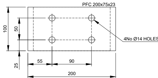
TPB-B-2 - PFC 200x75x23 Scale 1:5
