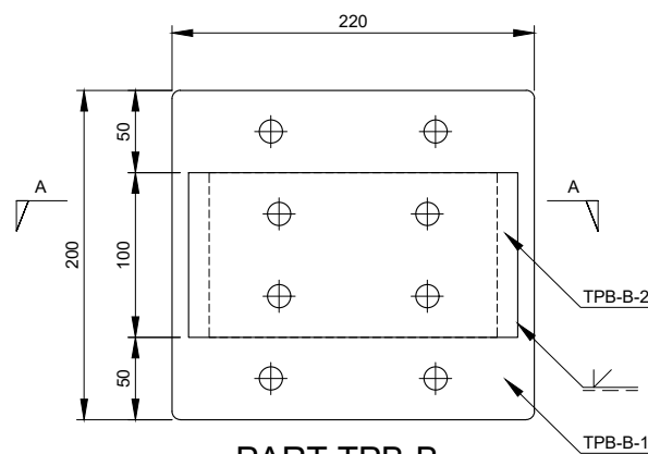
PART TPB-B Scale 1:5
