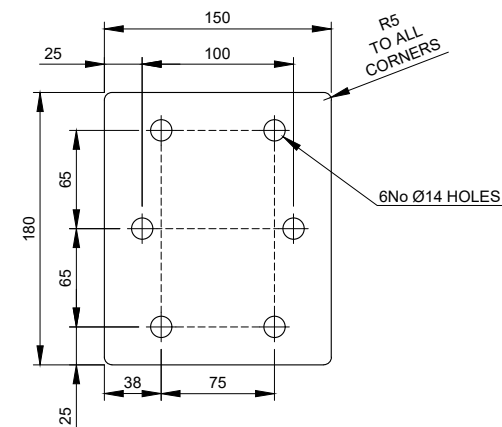
PART TPC-1 - 10mm THICK Scale 1:5
