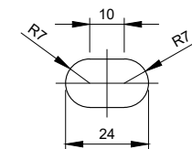
SLOTTED HOLE DETAIL Scale 1:2
