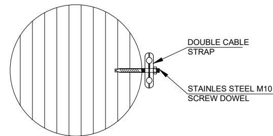
FEEDER MANAGEMENT Scale 1:10
