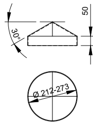
DETAIL A - LEAD CAP Scale 1:20
