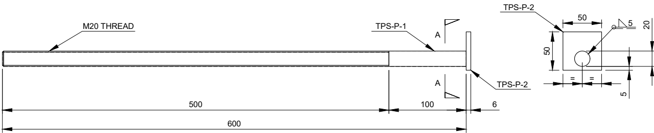
PART TPS-P Scale 1:5
