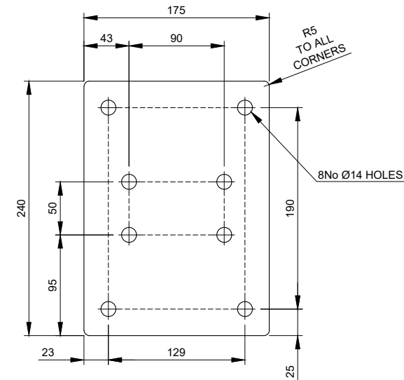
TPB-B-3 - 10mm THICK Scale 1:5
