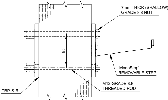
DETAIL E - REMOVABLE CLIMBING STEPS Scale 1:5
