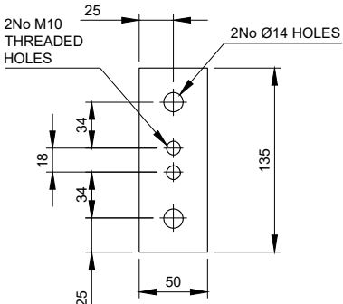
PART TPS-R Scale 1:5
